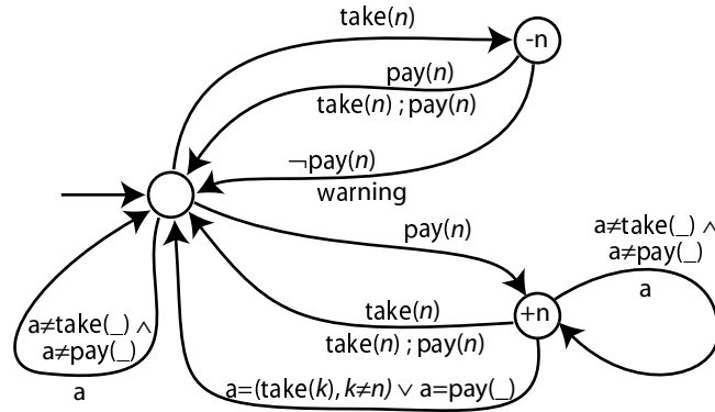
Figure 2: An edit automaton that effectively enforces the market policy.
