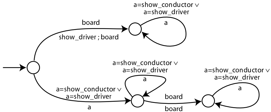
Figure 1: An insertion automaton that effectively enforces the cable-car policy on a uniform system.
