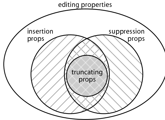
Figure 4: A taxonomy of effectively enforceable security properties on both uniform and nonuniform systems.
