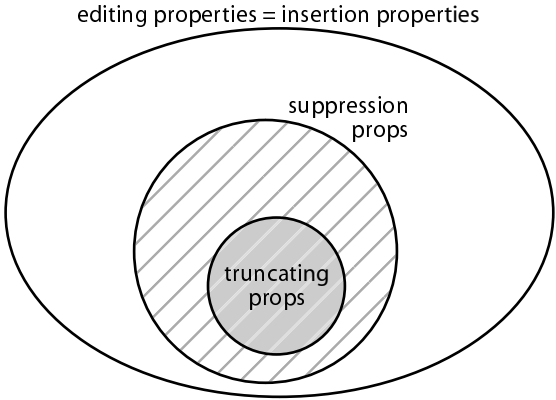
Figure 3: A taxonomy of precisely enforceable security properties on nonuniform systems.
