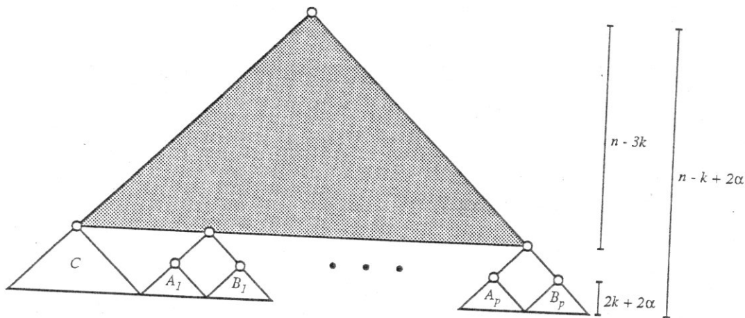
Figure 4.9: Schematic of the Floyd's Heapsort best case construction.
