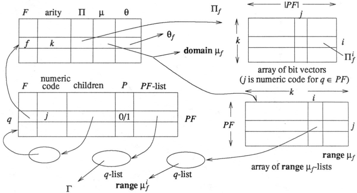
Fig.3. Core data structure
