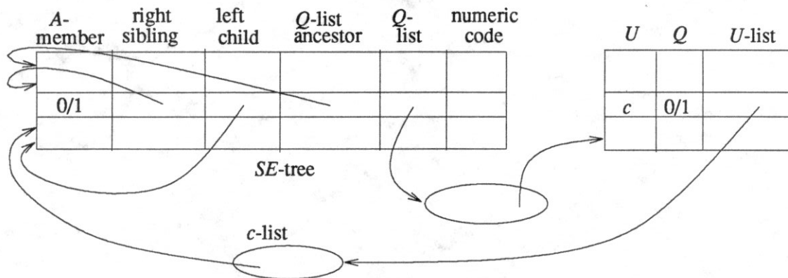
Fig.1. SE-structure( U, A, Q )
