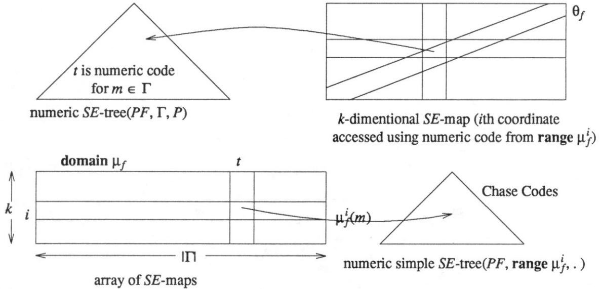
Fig.4. Data structure for \theta_f and \mu_f^i
