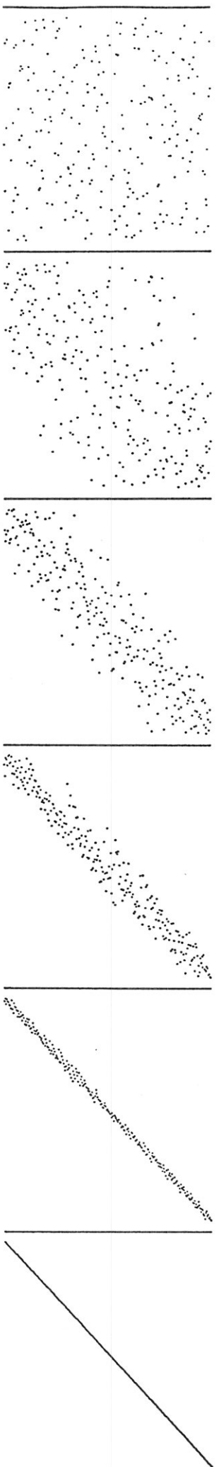
Figure 3. Shellsort
