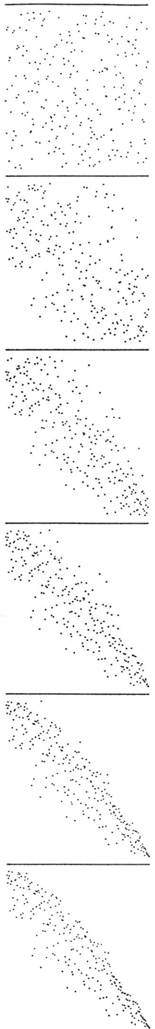
Figure 2. Dobosiewicz's variant
