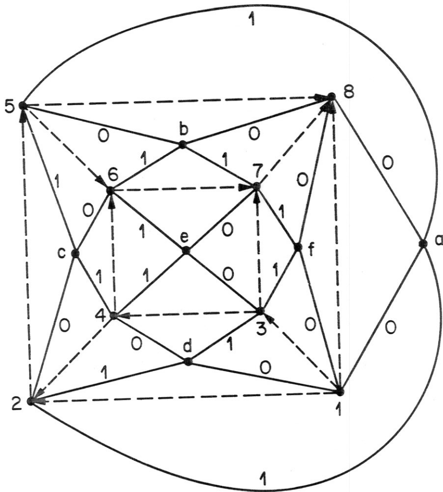
Figure 4. The angle graph of the graph in Figure 1(a), with the original graph indicated by dashed lines. A bipolar orientation and the corresponding bipolar marking are shown.
